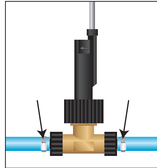
6. Tighten the hose clamps so the hose is secured to the adapters. NOTICE: Be sure it can't leak any water.
